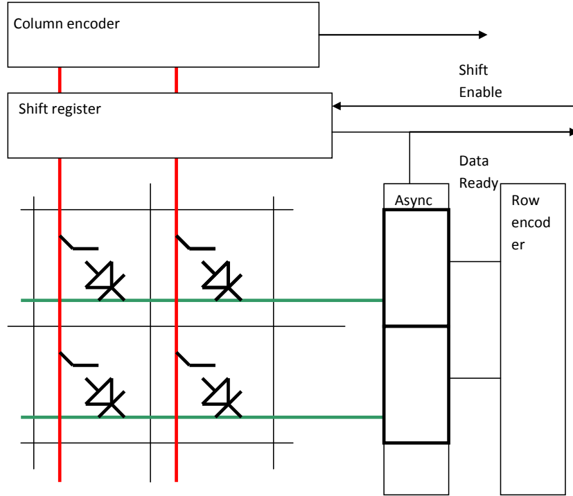
Figure 4: fast scan conceptual pixel array.
