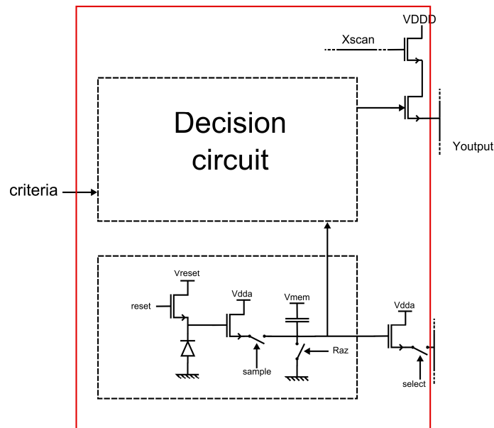
Figure 5: Fast scan pixel.
